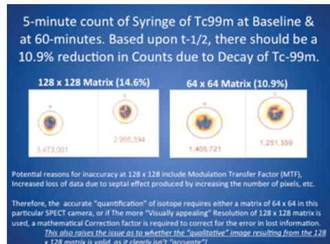
Figure 2: “Quantitative” Calibration of Nuclear Camera using TFM®.
