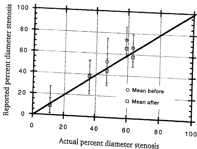
Figure 4. Percent diameter stenosis read from photographic reproductions of 5 stenotic arteries ranging from 11% to 63%. Results of the readings before (open circles) and after (open squares) training (y-axis) are plotted against actual percent diameter stenosis displayed on the x-axis. While improvement was noted in 80% of the cases, no statistical differences occurred since edges were outlined both before and after training, excluding edge detection as a potential problem.
