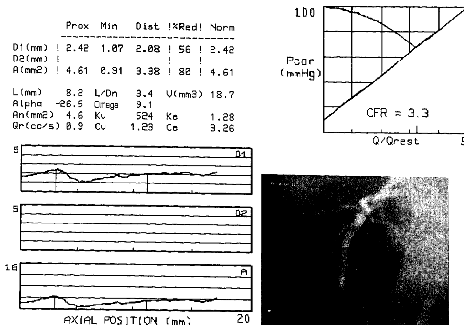
Figure 1. Automated quantitative coronary arteriography in a subject with a 56% diameter stenosis of a diagonal branch of the left anterior descending coronary artery. The artery is bordered by a broken line, which defines the region of maximal stenosis. Other information shown includes an 80% reduction in area, entry (alpha) and exit (omega) angles to and from the lesion, and the coronary flow reserve. A = cross-luminal area; An = normal cross-sectional area; CFR = calculated coronary (stenosis) flow reserve; Ce and Ke = momentum coefficient losses based on alpha and omega; Cv and Kv = coefficients of viscosity losses secondary to geometry of stenosis; D 1 and D 2 = orthogonal single-plane diameters; Dist = distal; L = lesion length; L/Dn = length/diameter ratio; Min = minimal diameter; Norm = normal coronary segment; Pcor = coronary perfusion pressure; %Red = percent reduction; Prox = proximal segment; Q/Q rest = ratio of maximal to rest flow or coronary flow reserve; Qr = rest flow; V = intraluminal volume in the stenotic segment.
