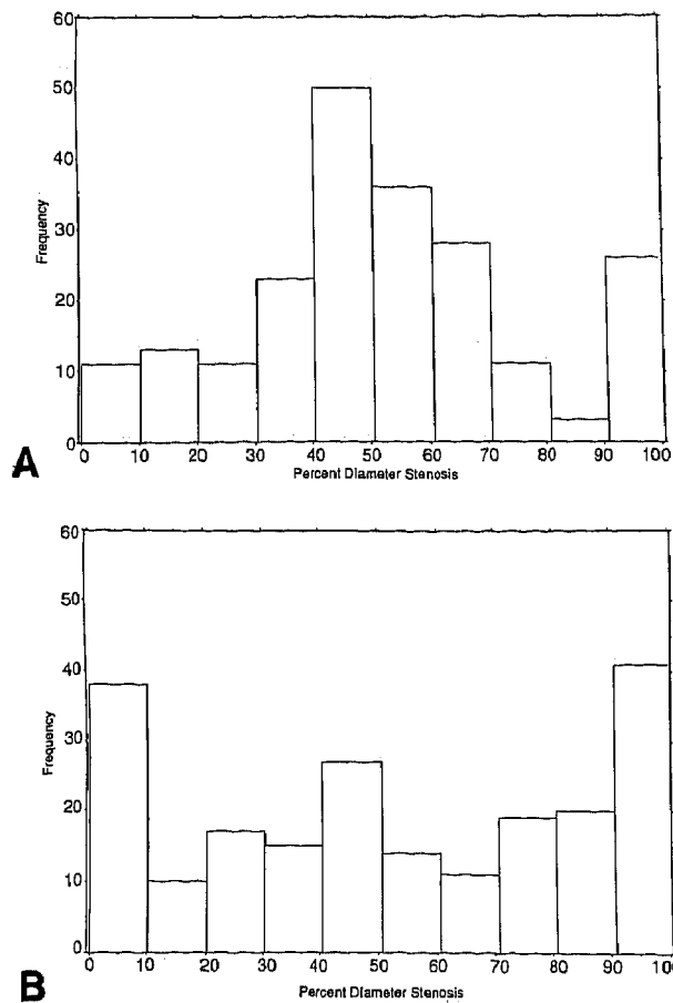
Figure 4. A, Frequency histogram of percent diameter stenosis as measured by quantitative coronary arteriography. (A) and the visual method (B). A, The bar graph shows a gaussian type distribution of disease over the 212 coronary artery segments studied. A significant number of arteries are totally occluded, reflecting the high prevalence of disease in the patients examined. B, The bar graph represents three distinct peaks at 0%, 50% and 100% diameter stenosis. Detection of disease between the peaks is less frequent and is found at 10% intervals. Visual reporting of percent diameter stenosis is trimodal and not gaussian.
