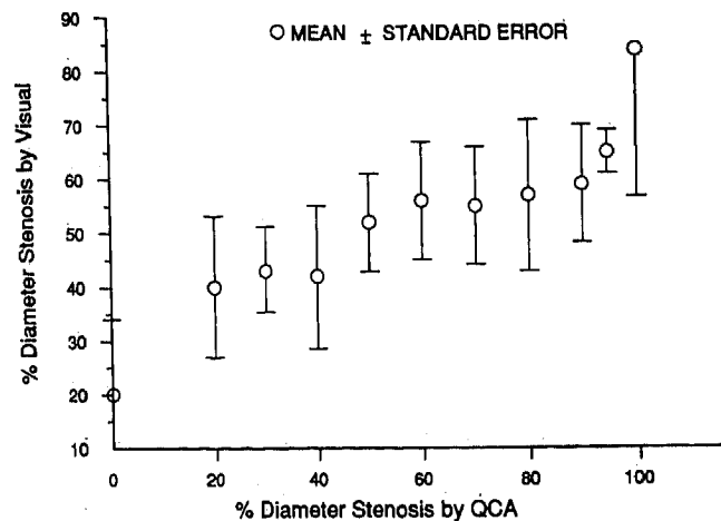
Figure 5. Percent diameter stenosis by the visual method plotted against percent diameter stenosis by quantitative coronary arteriography (QCA). There is good agreement between the two methods at 0% and 100% diameter stenosis. However, visual estimates tend to cluster disease between 40% and 60% (50% peak) when quantitative coronary arteriography (QCA) reports percent diameter stenosis ranging from 20% to 80%.
